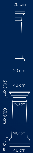
Art. 2289 h 101 cm
